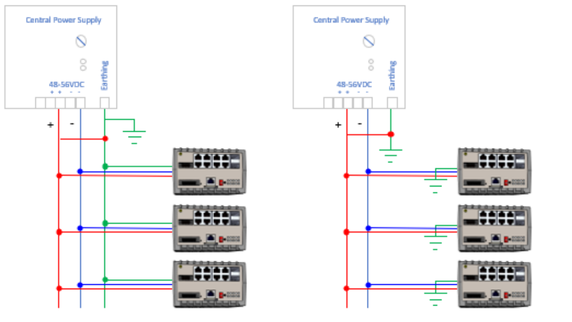
Examples of unauthorized grounding configurations. These configuration examples show the unsuitable and not allowed grounding schema, which leads to potential entanglement and short-circuit. The minus pole must never be connected to the grounding connection.
