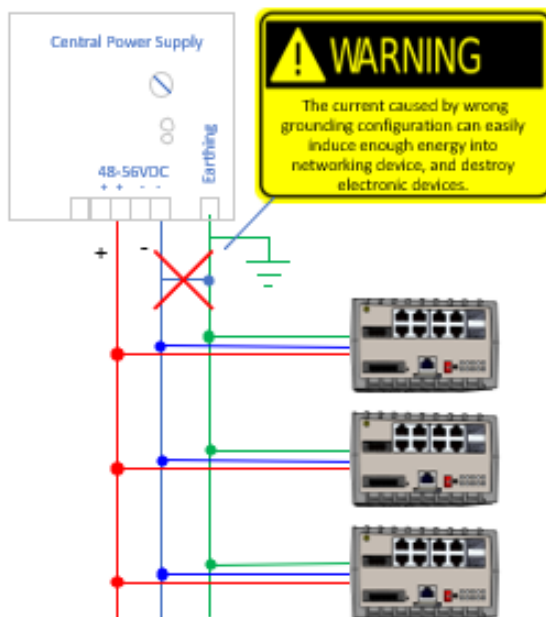
Examples of unauthorized grounding configurations. These configuration examples show the unsuitable and not allowed grounding schema, which leads to potential entanglement and short-circuit. The minus pole must never be connected to the grounding connection.
