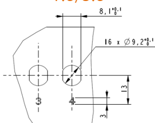
Coax. 1.6/5.6
